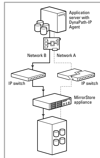
3 Traffic fails over to Network B without data loss.
