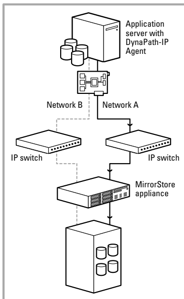
1 Normal traffic flows on Network A. Status packets peer deep into the network to identify faults.
